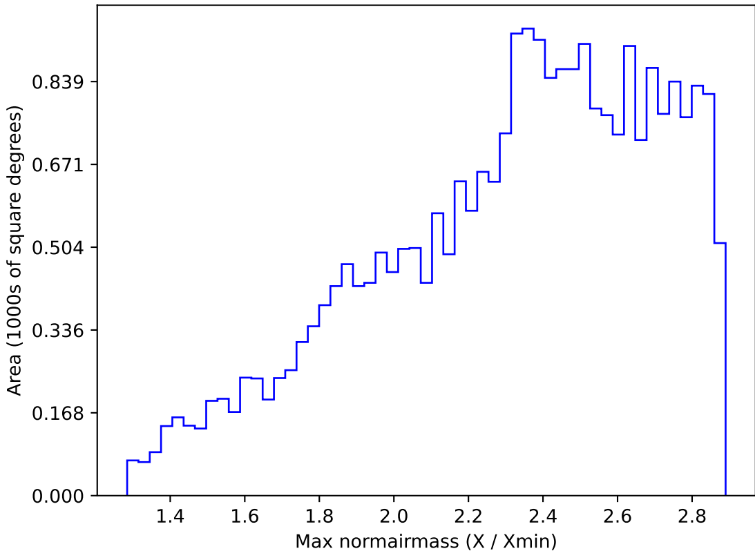
no_high_blob_v3.3_10yrs All sky all bands: Max normairmass
