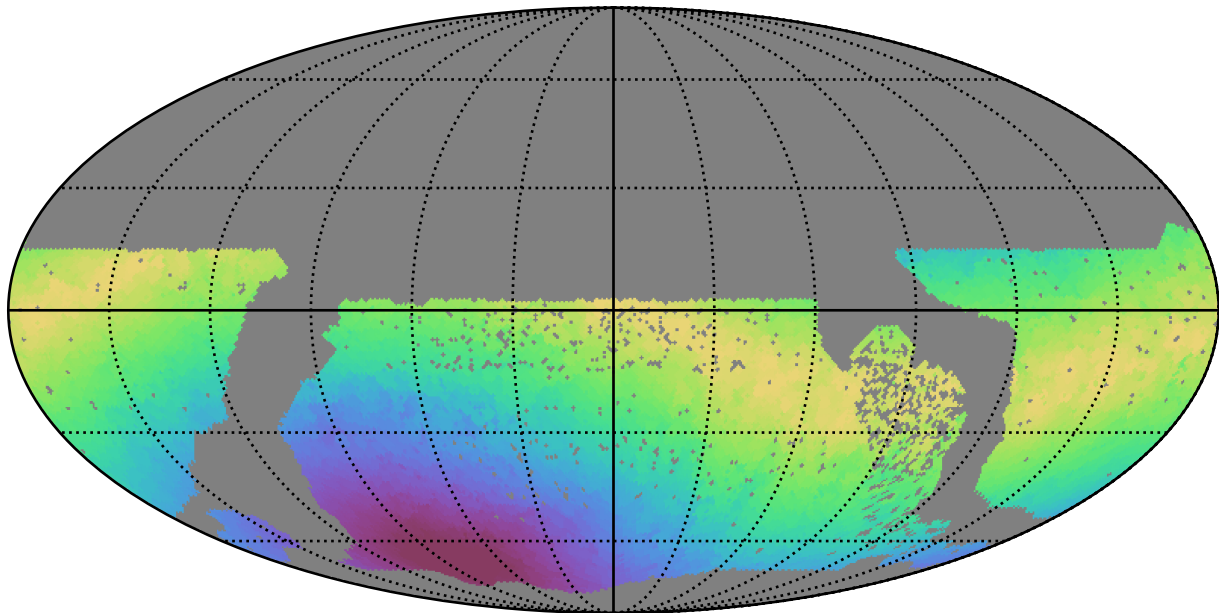
no_high_blob_v3.3_10yrs WFD z band: Max moonDistance
