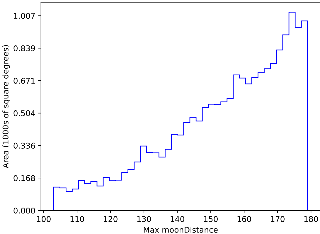
no_high_blob_v3.3_10yrs WFD z band: Max moonDistance
