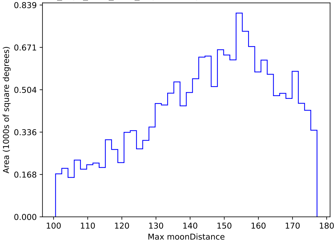
no_high_blob_v3.3_10yrs WFD y band: Max moonDistance
