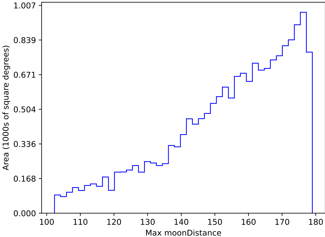
no_high_blob_v3.3_10yrs WFD u band: Max moonDistance
