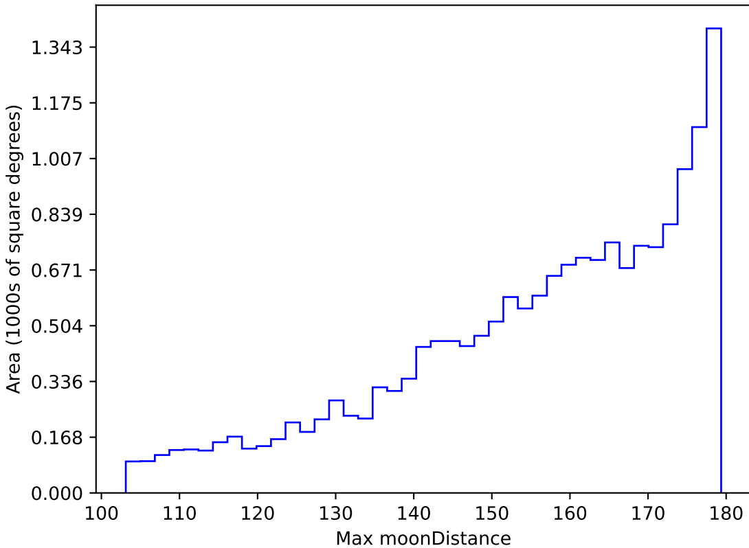
no_high_blob_v3.3_10yrs WFD r band: Max moonDistance
