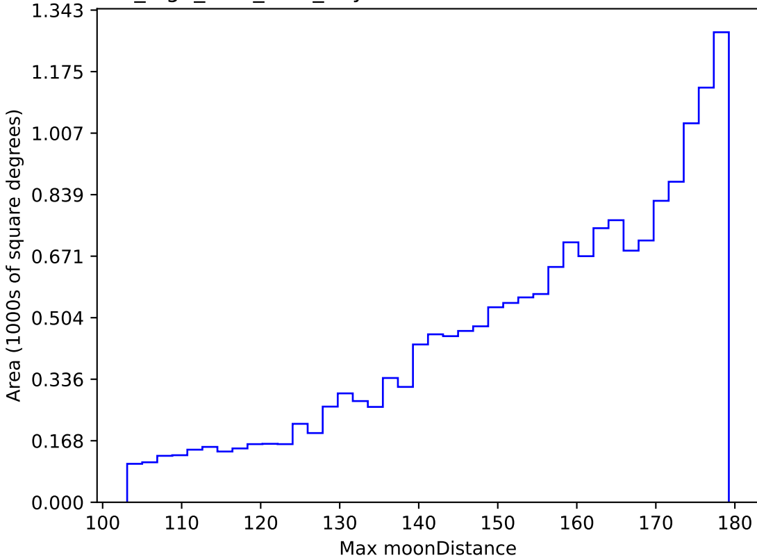
no_high_blob_v3.3_10yrs WFD i band: Max moonDistance
