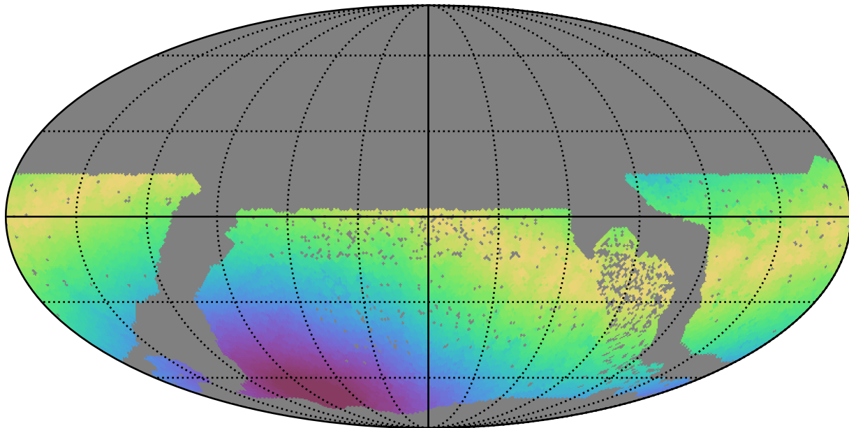
no_high_blob_v3.3_10yrs WFD g band: Max moonDistance
