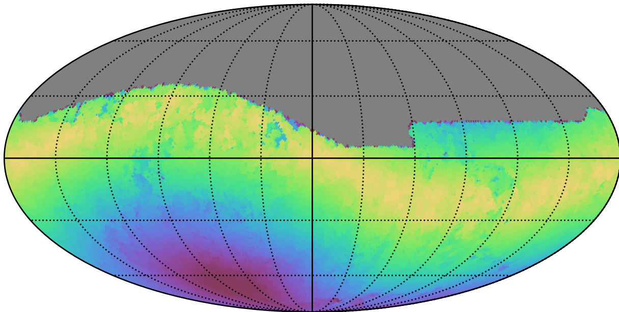
no_high_blob_v3.3_10yrs All sky z band: Max moonDistance
