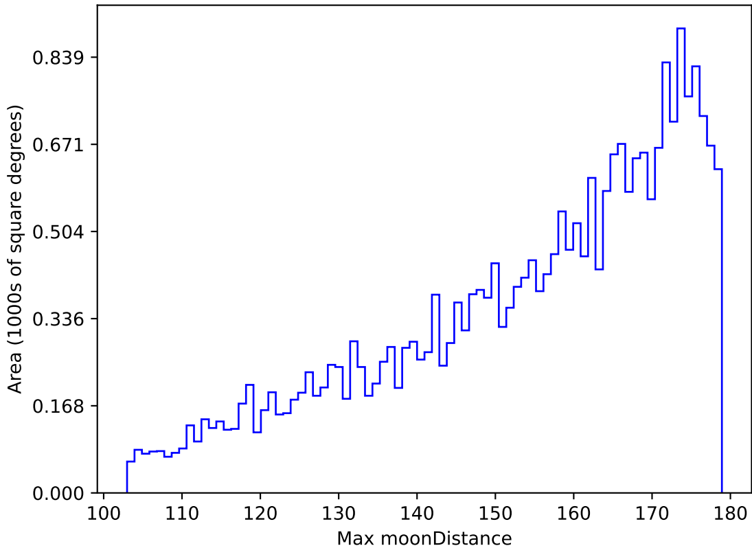
no_high_blob_v3.3_10yrs All sky z band: Max moonDistance
