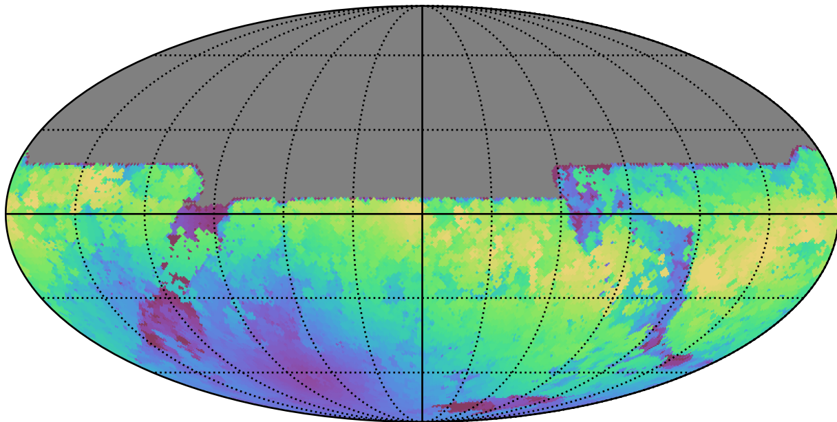
no_high_blob_v3.3_10yrs All sky y band: Max moonDistance
