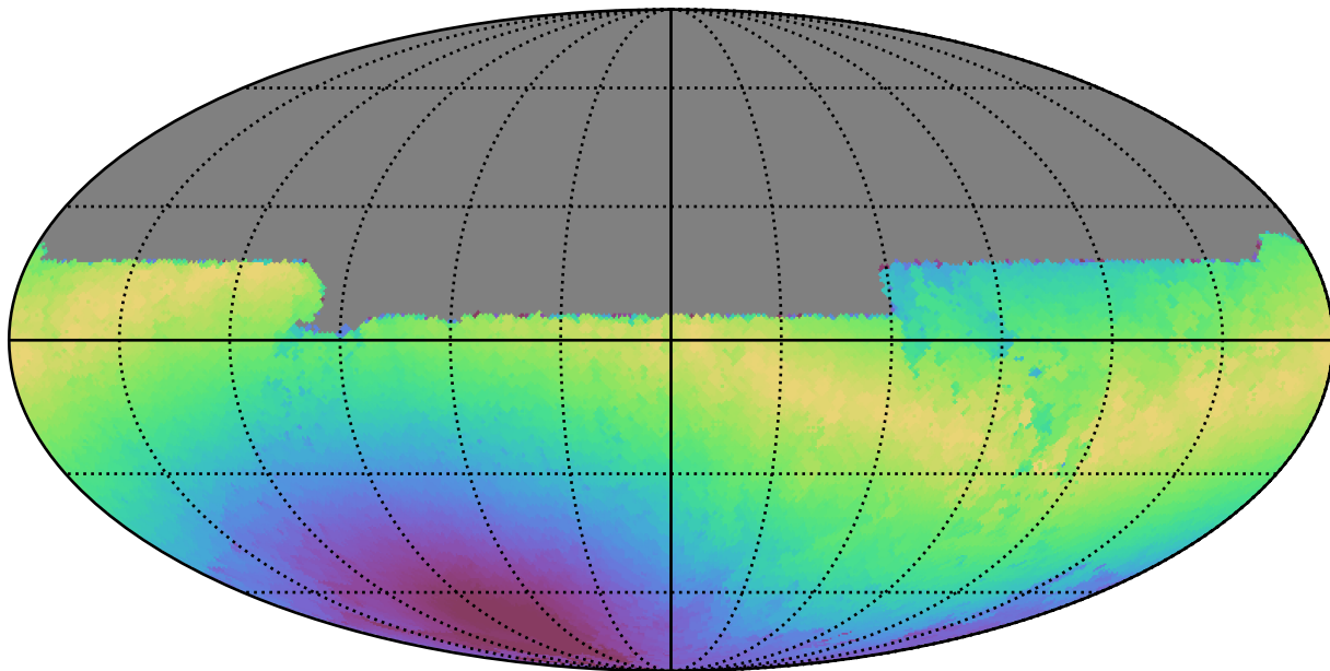
no_high_blob_v3.3_10yrs All sky u band: Max moonDistance
