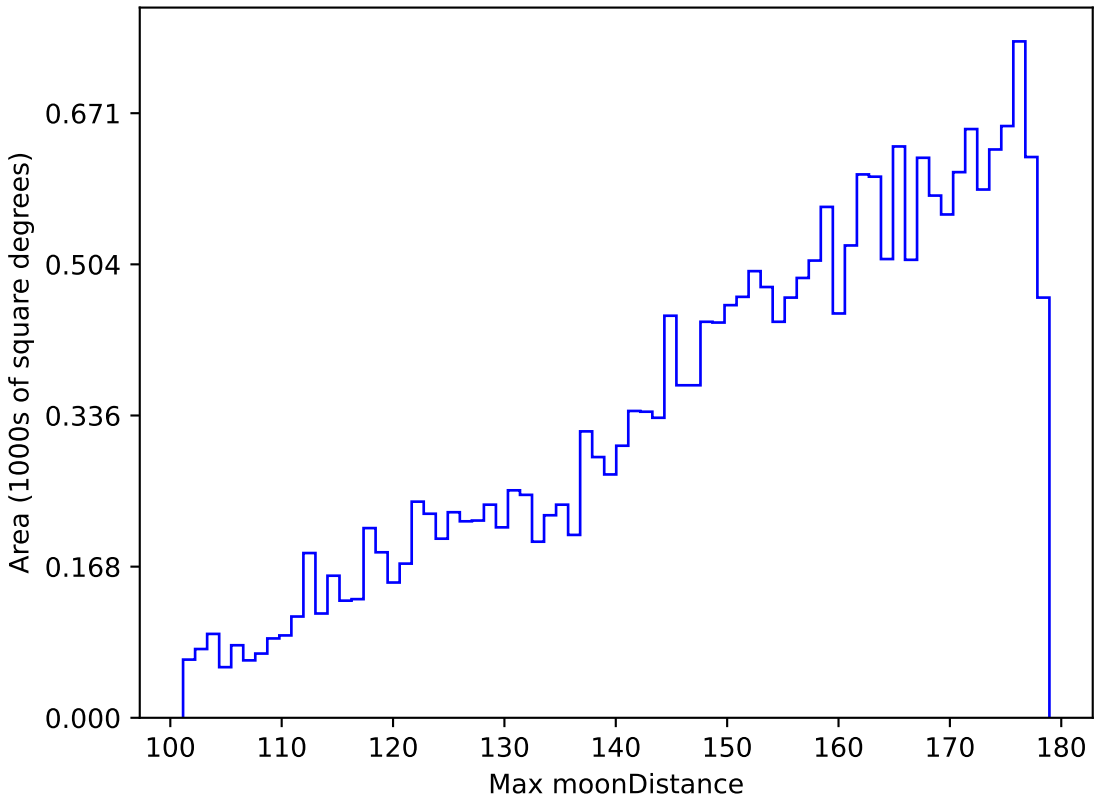
no_high_blob_v3.3_10yrs All sky u band: Max moonDistance
