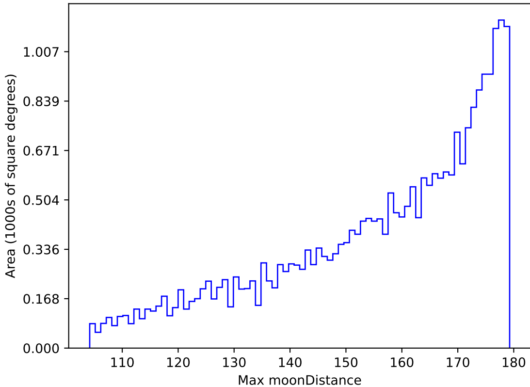
no_high_blob_v3.3_10yrs All sky r band: Max moonDistance
