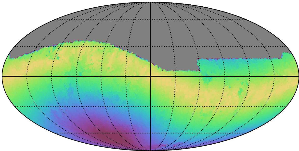
no_high_blob_v3.3_10yrs All sky i band: Max moonDistance
