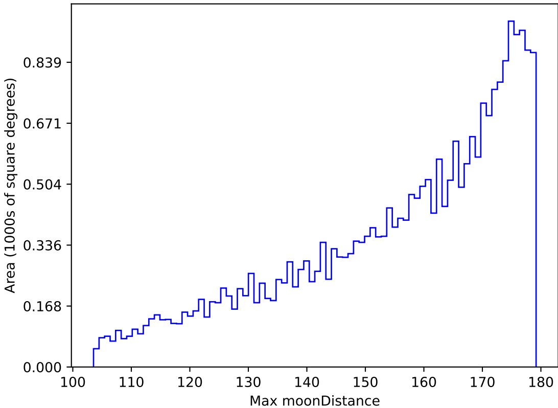
no_high_blob_v3.3_10yrs All sky i band: Max moonDistance
