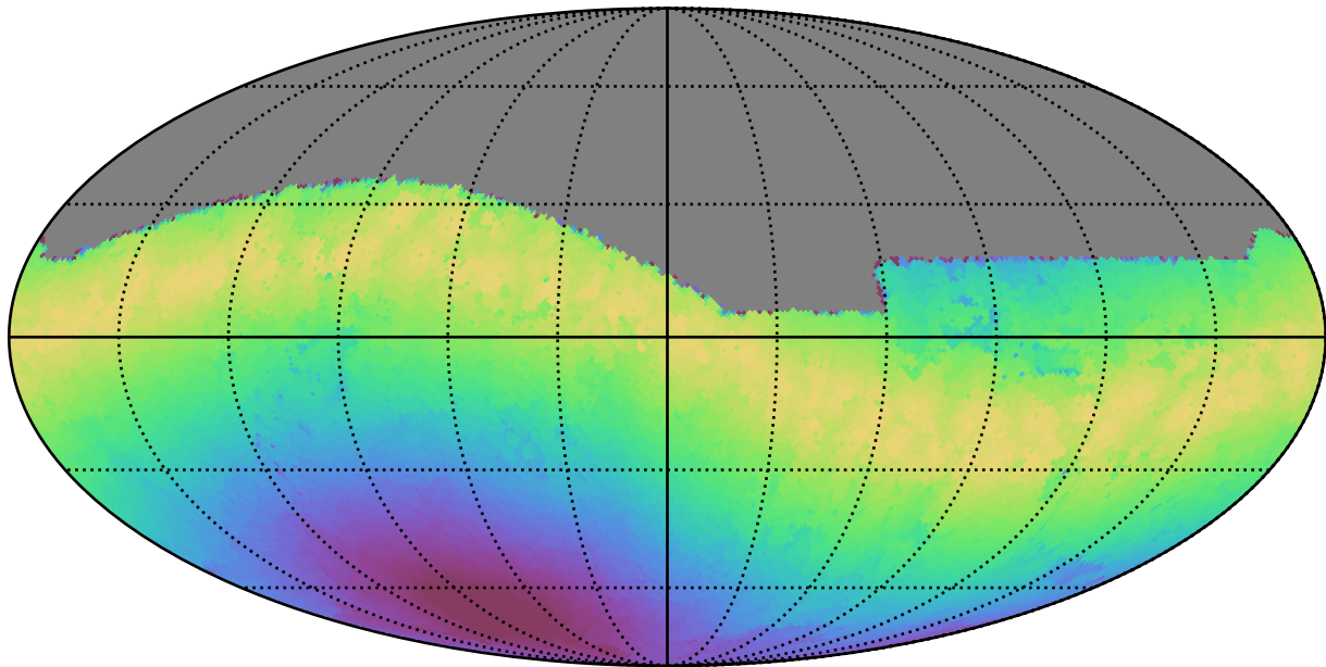
no_high_blob_v3.3_10yrs All sky g band: Max moonDistance
