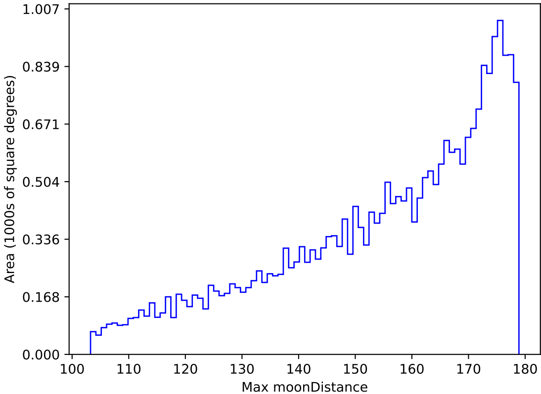
no_high_blob_v3.3_10yrs All sky g band: Max moonDistance
