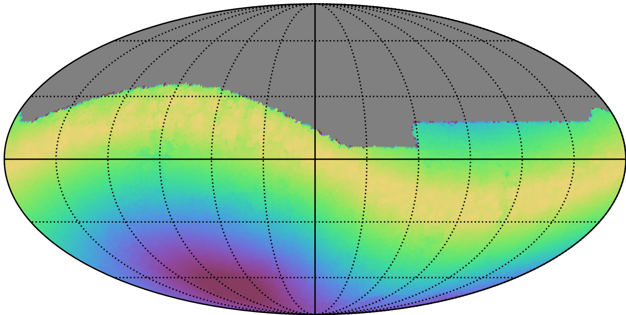
no_high_blob_v3.3_10yrs All sky all bands: Max moonDistance
