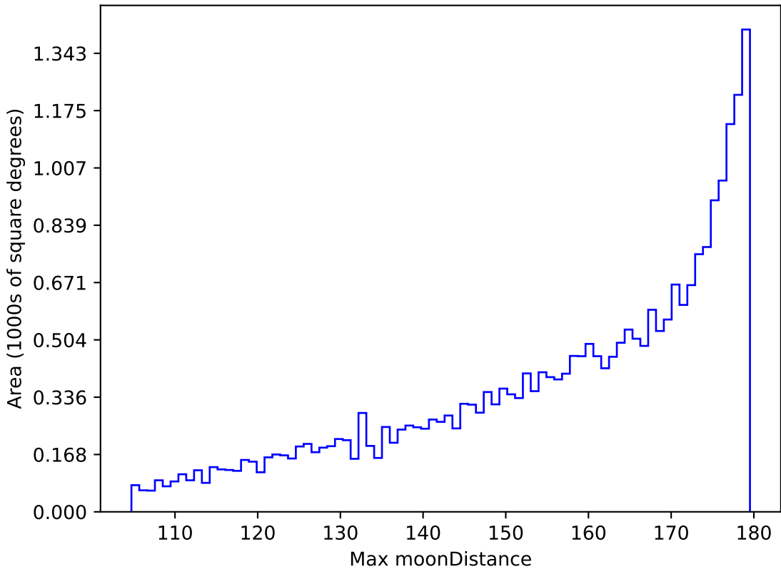
no_high_blob_v3.3_10yrs All sky all bands: Max moonDistance
