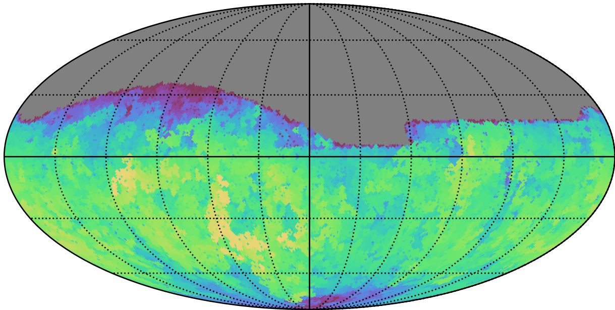
no_high_blob_v3.3_10yrs Yr 1 all bands: Max fiveSigmaDepth
