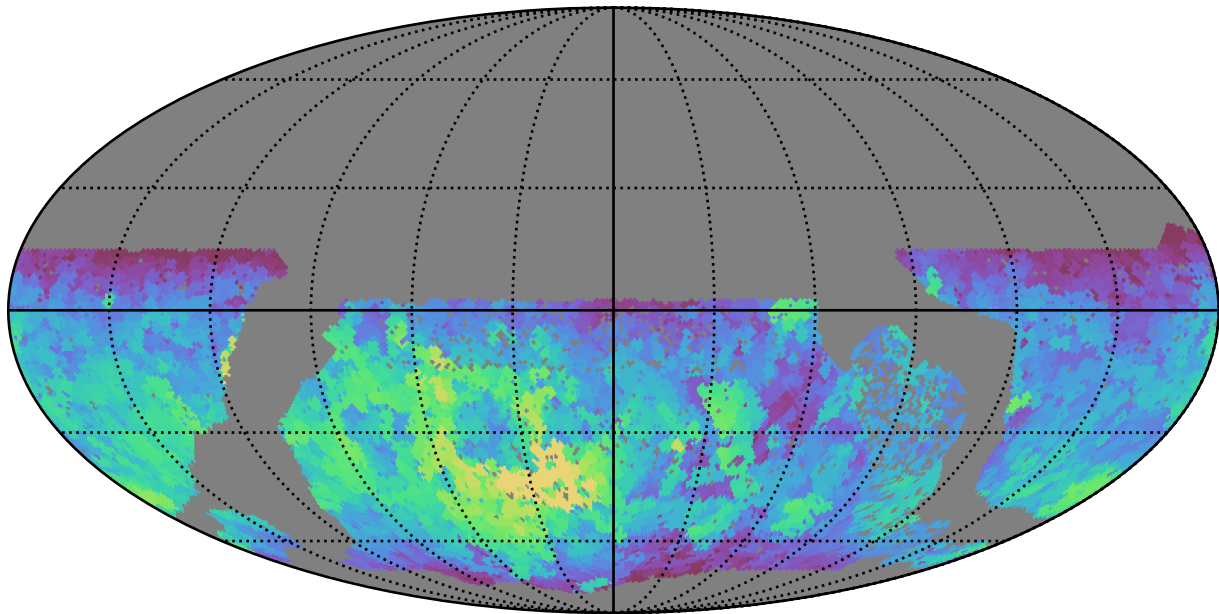
no_high_blob_v3.3_10yrs WFD all bands: Max fiveSigmaDepth
