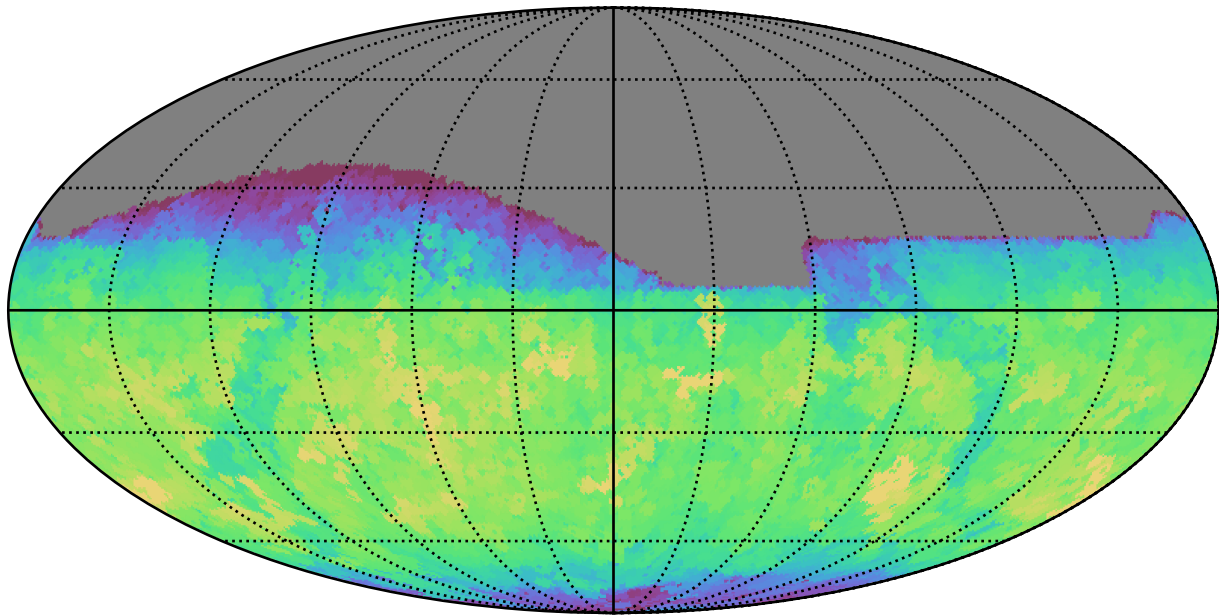
no_high_blob_v3.3_10yrs All sky z band: Max fiveSigmaDepth
