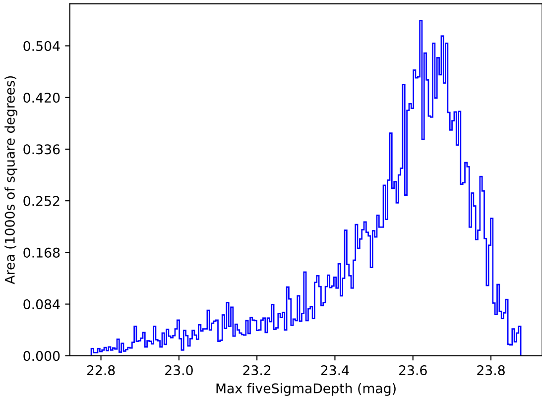
no_high_blob_v3.3_10yrs All sky z band: Max fiveSigmaDepth
