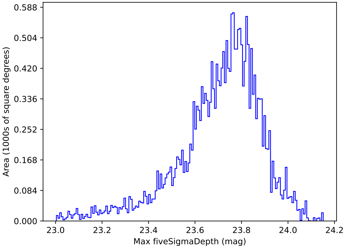
no_high_blob_v3.3_10yrs All sky u band: Max fiveSigmaDepth
