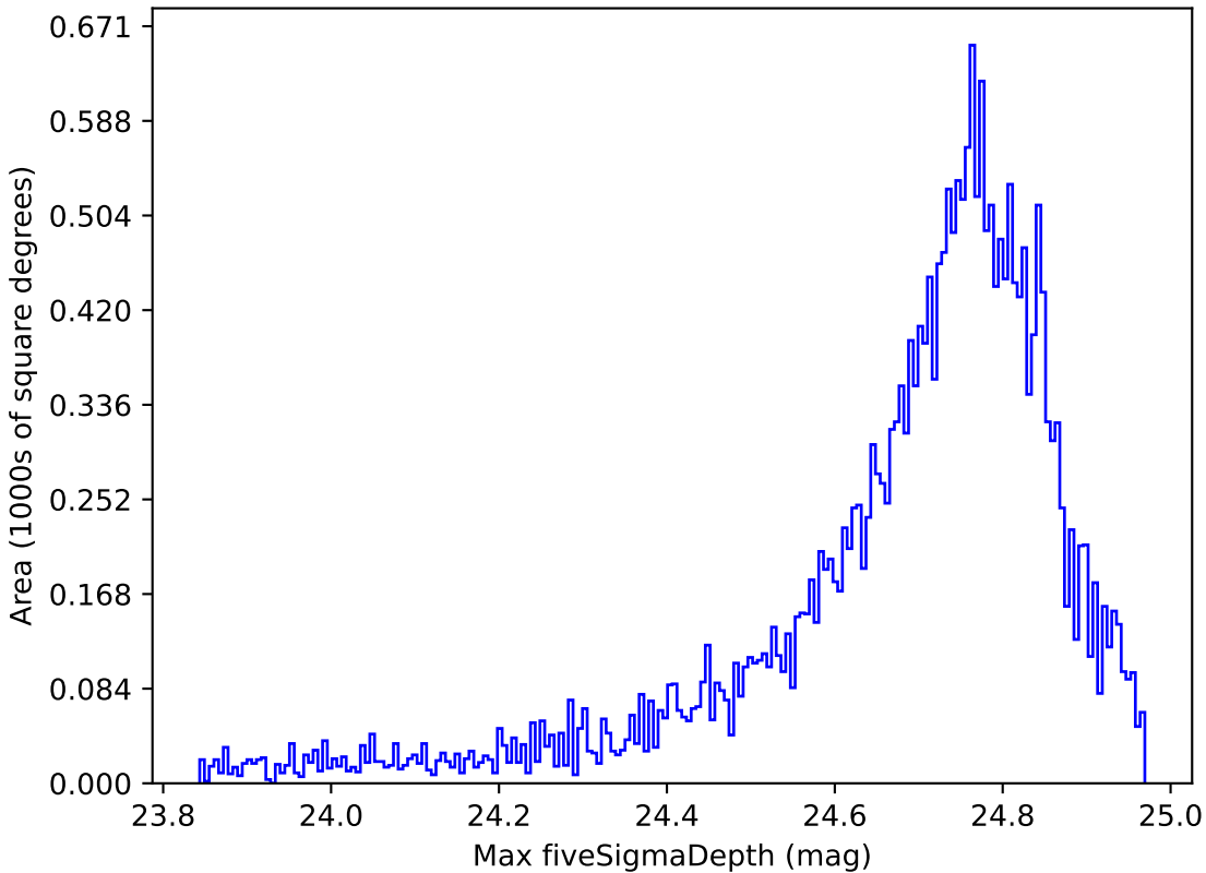
no_high_blob_v3.3_10yrs All sky r band: Max fiveSigmaDepth
