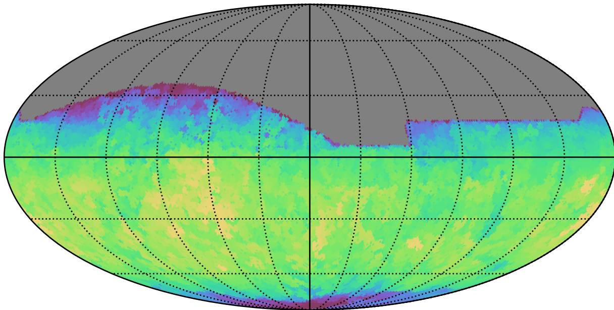
no_high_blob_v3.3_10yrs All sky i band: Max fiveSigmaDepth
