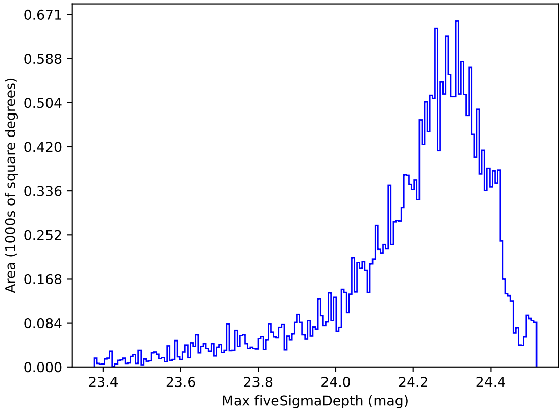
no_high_blob_v3.3_10yrs All sky i band: Max fiveSigmaDepth
