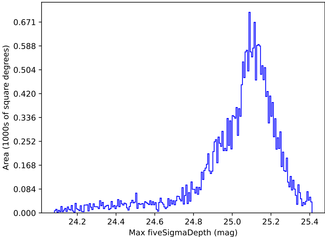
no_high_blob_v3.3_10yrs All sky g band: Max fiveSigmaDepth
