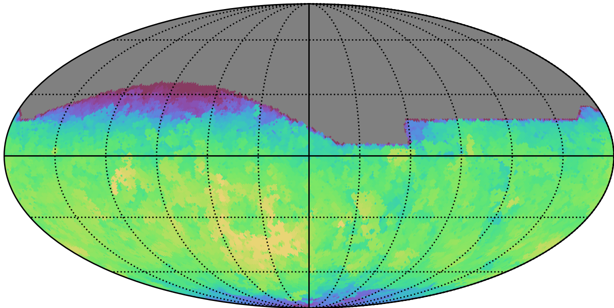
no_high_blob_v3.3_10yrs All sky all bands: Max fiveSigmaDepth
