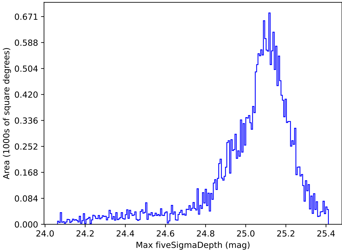
no_high_blob_v3.3_10yrs All sky all bands: Max fiveSigmaDepth
