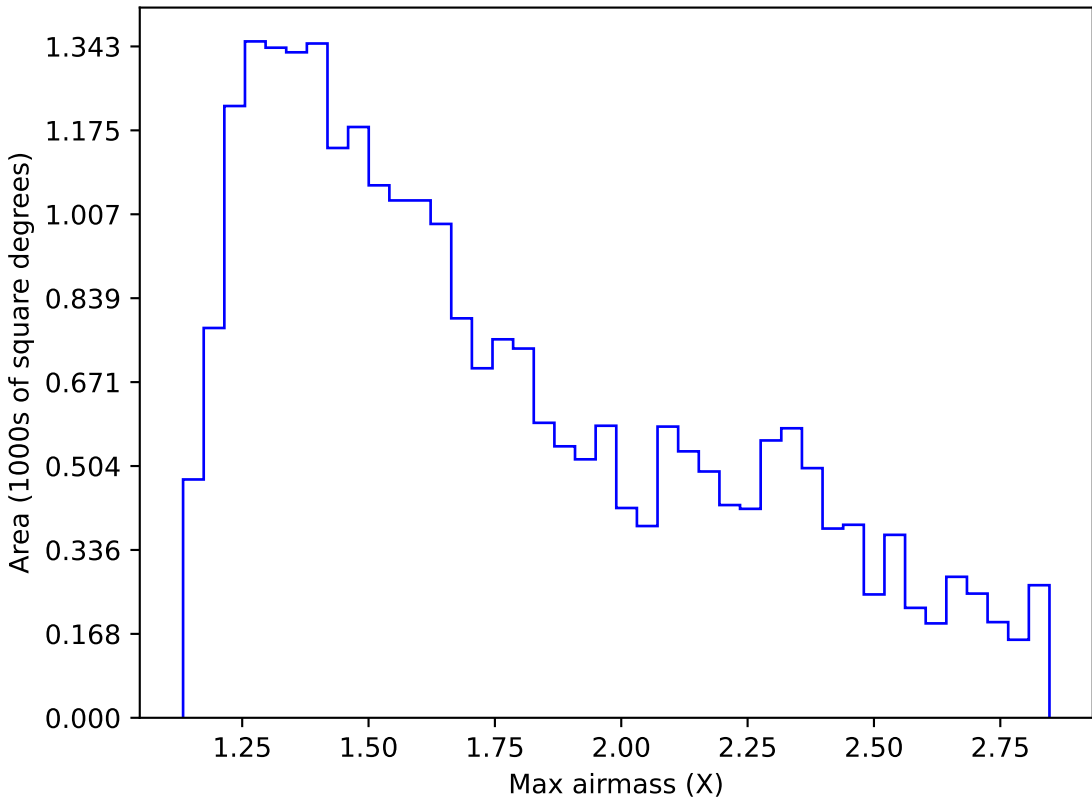
no_high_blob_v3.3_10yrs Yr 1 z band: Max airmass
