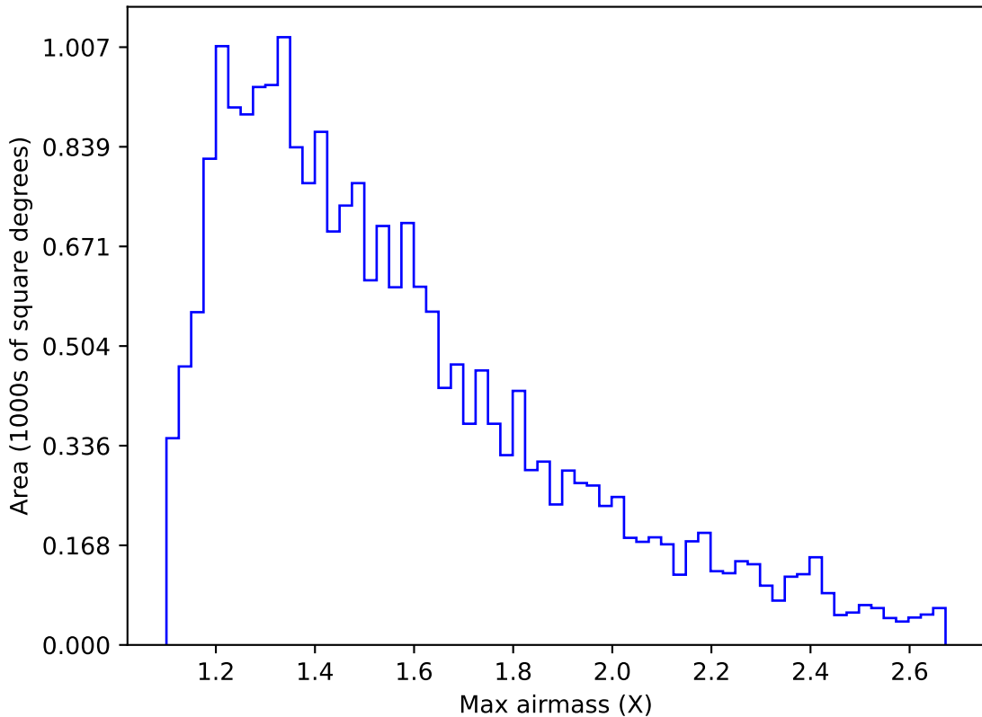
no_high_blob_v3.3_10yrs Yr 1 u band: Max airmass
