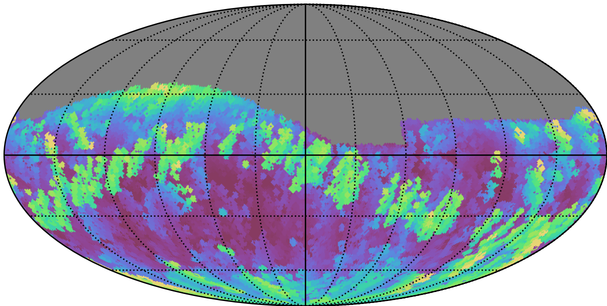
no_high_blob_v3.3_10yrs Yr 1 r band: Max airmass
