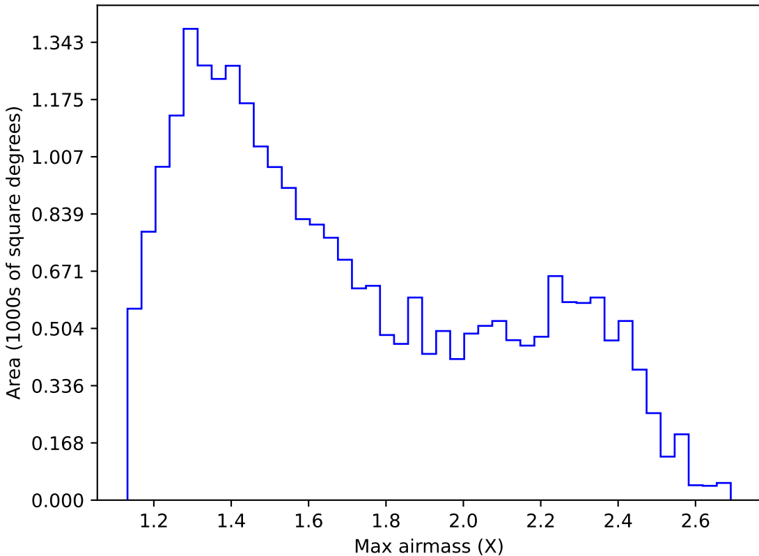
no_high_blob_v3.3_10yrs Yr 1 r band: Max airmass
