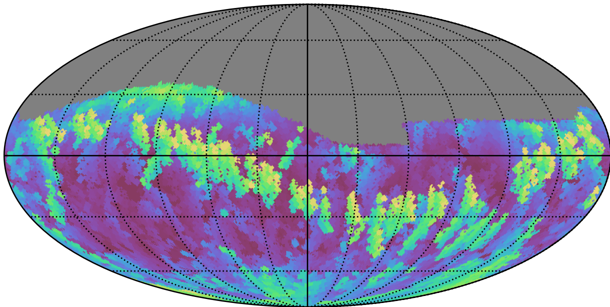
no_high_blob_v3.3_10yrs Yr 1 i band: Max airmass
