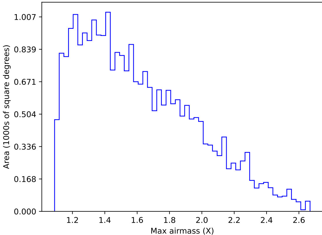
no_high_blob_v3.3_10yrs Yr 1 g band: Max airmass
