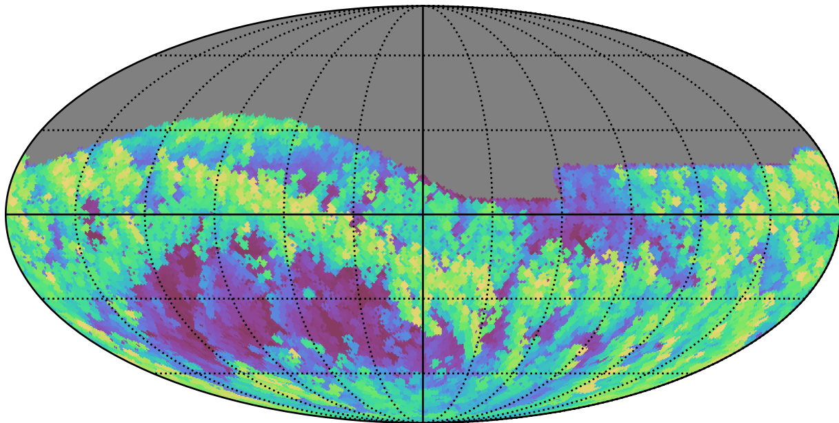
no_high_blob_v3.3_10yrs Yr 1 all bands: Max airmass
