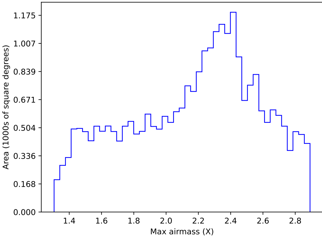
no_high_blob_v3.3_10yrs Yr 1 all bands: Max airmass
