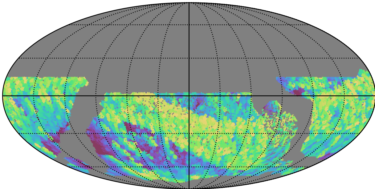
no_high_blob_v3.3_10yrs WFD z band: Max airmass
