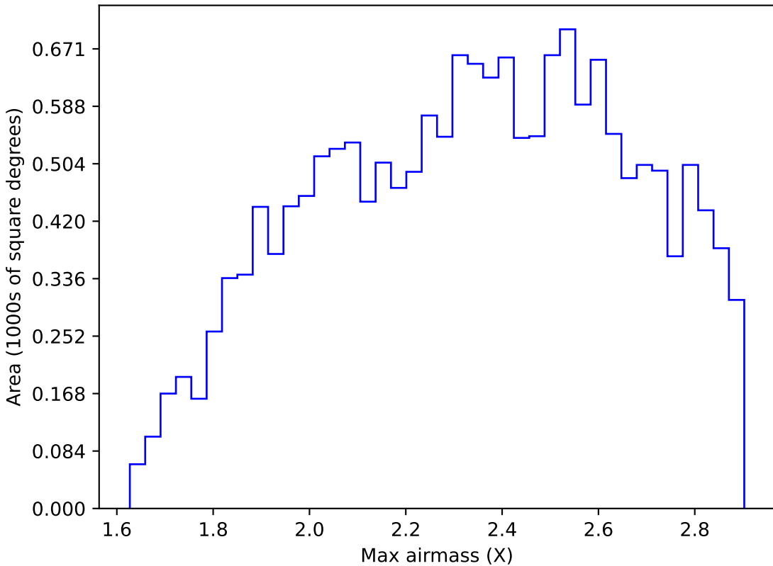
no_high_blob_v3.3_10yrs WFD y band: Max airmass
