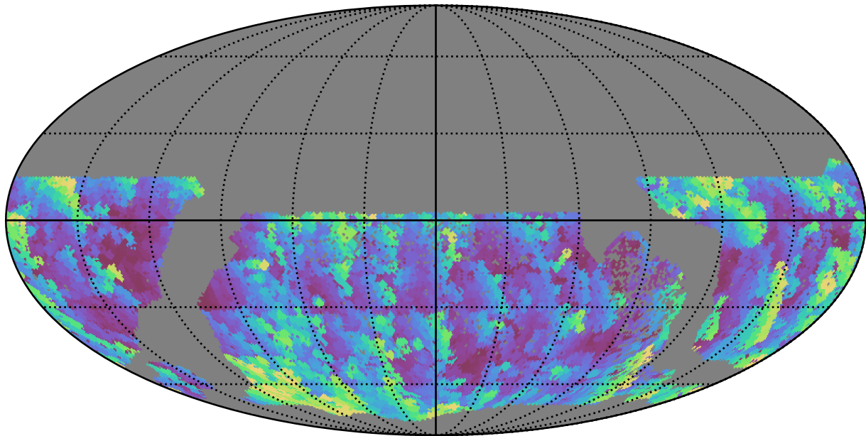
no_high_blob_v3.3_10yrs WFD u band: Max airmass
