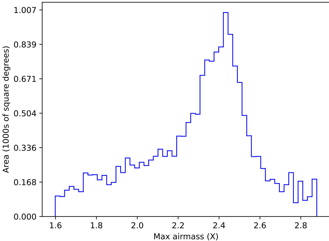
no_high_blob_v3.3_10yrs WFD r band: Max airmass
