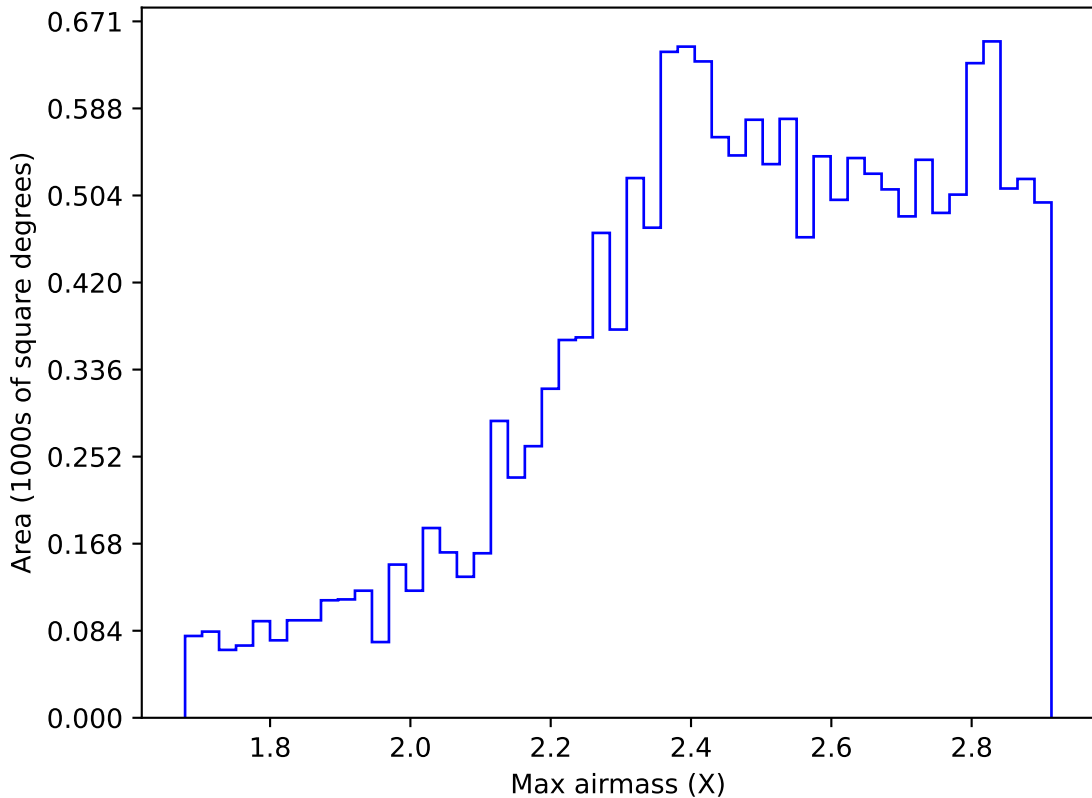
no_high_blob_v3.3_10yrs WFD i band: Max airmass
