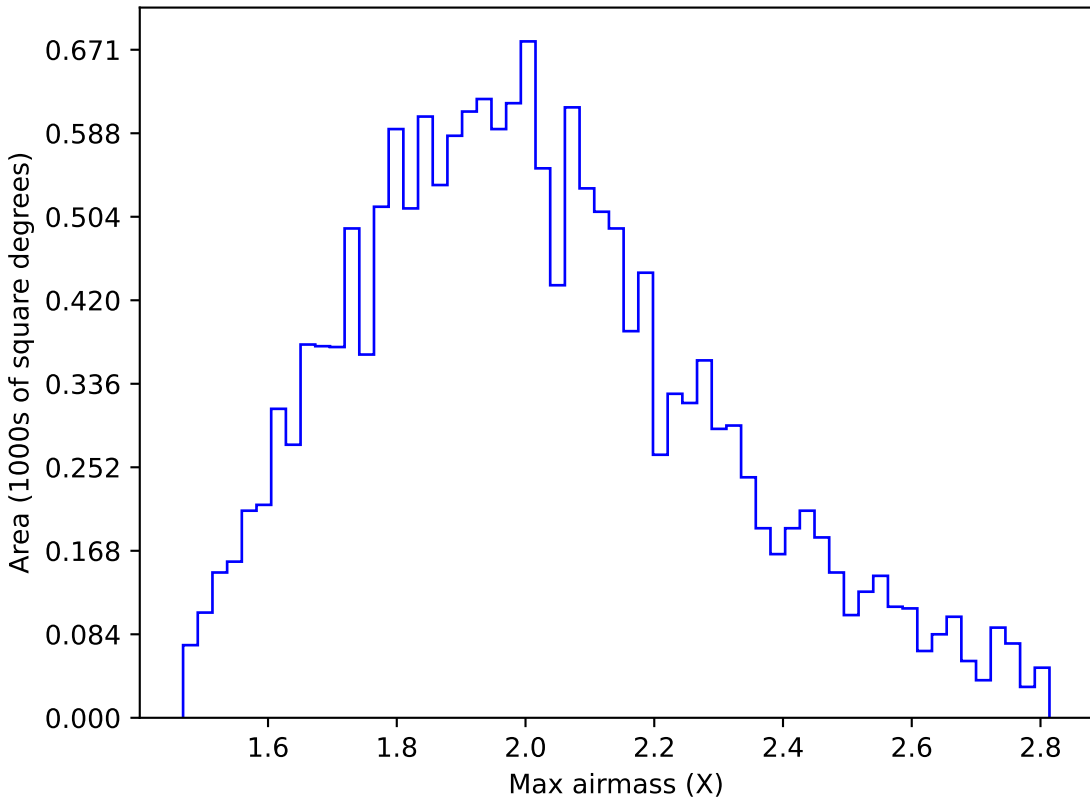
no_high_blob_v3.3_10yrs WFD g band: Max airmass
