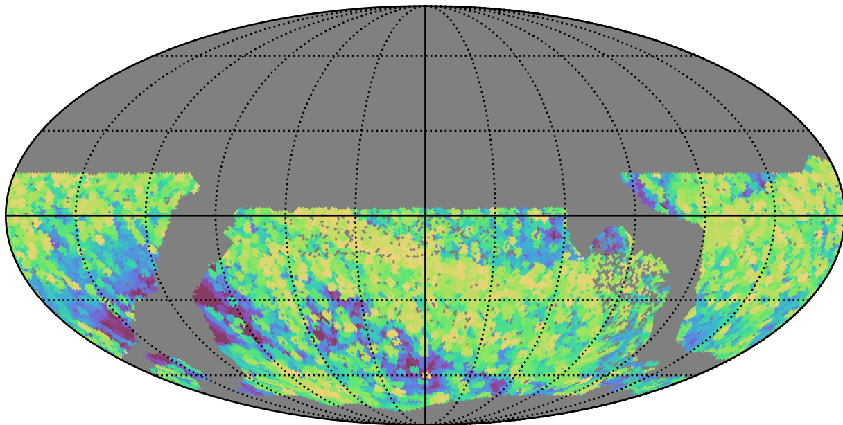
no_high_blob_v3.3_10yrs WFD all bands: Max airmass
