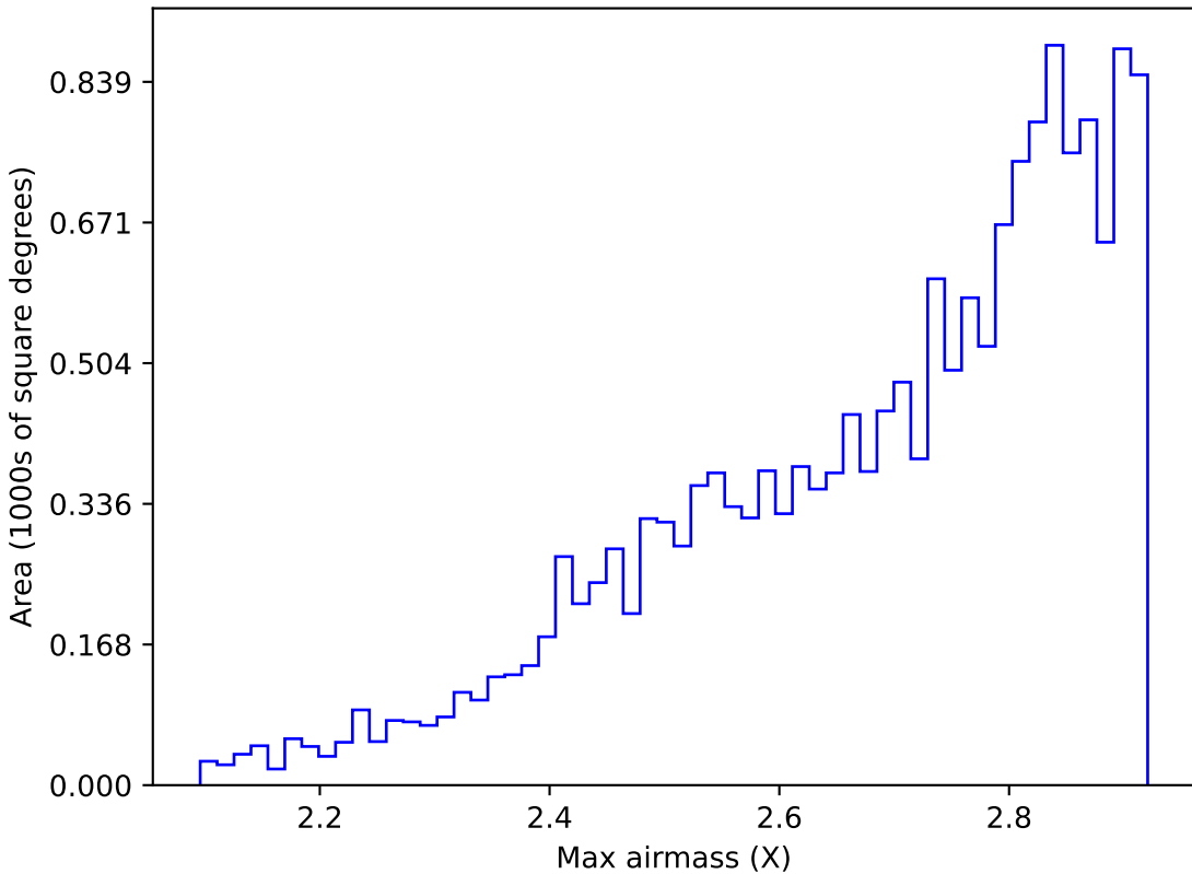
no_high_blob_v3.3_10yrs WFD all bands: Max airmass
