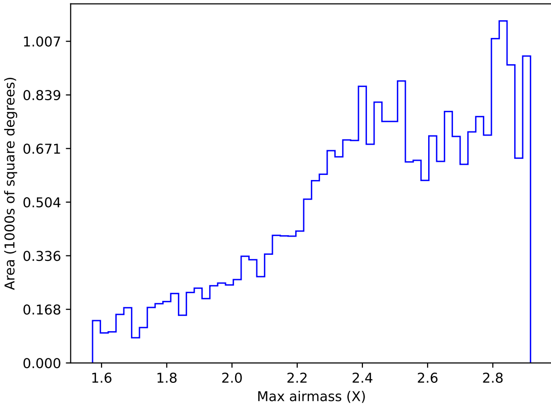
no_high_blob_v3.3_10yrs All sky z band: Max airmass
