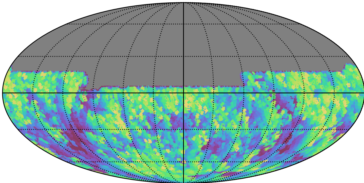
no_high_blob_v3.3_10yrs All sky y band: Max airmass
