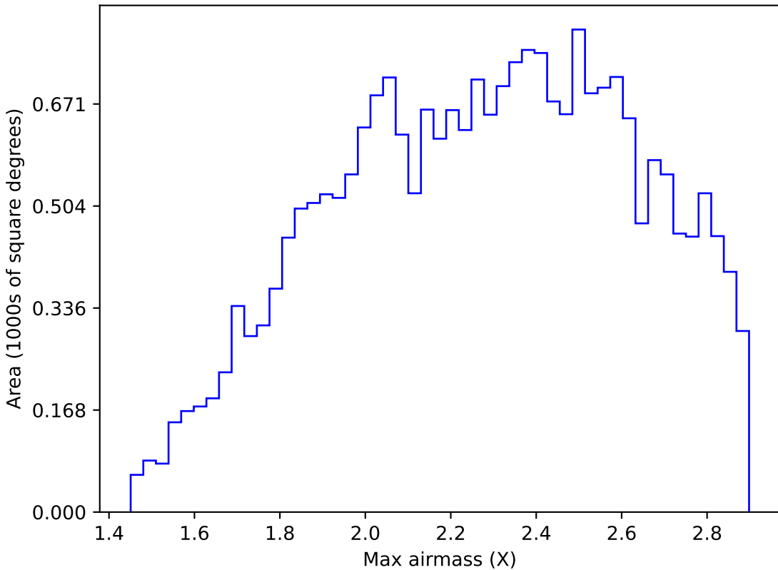
no_high_blob_v3.3_10yrs All sky y band: Max airmass
